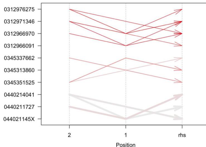
Parallel coordinates plot for 12 rules
