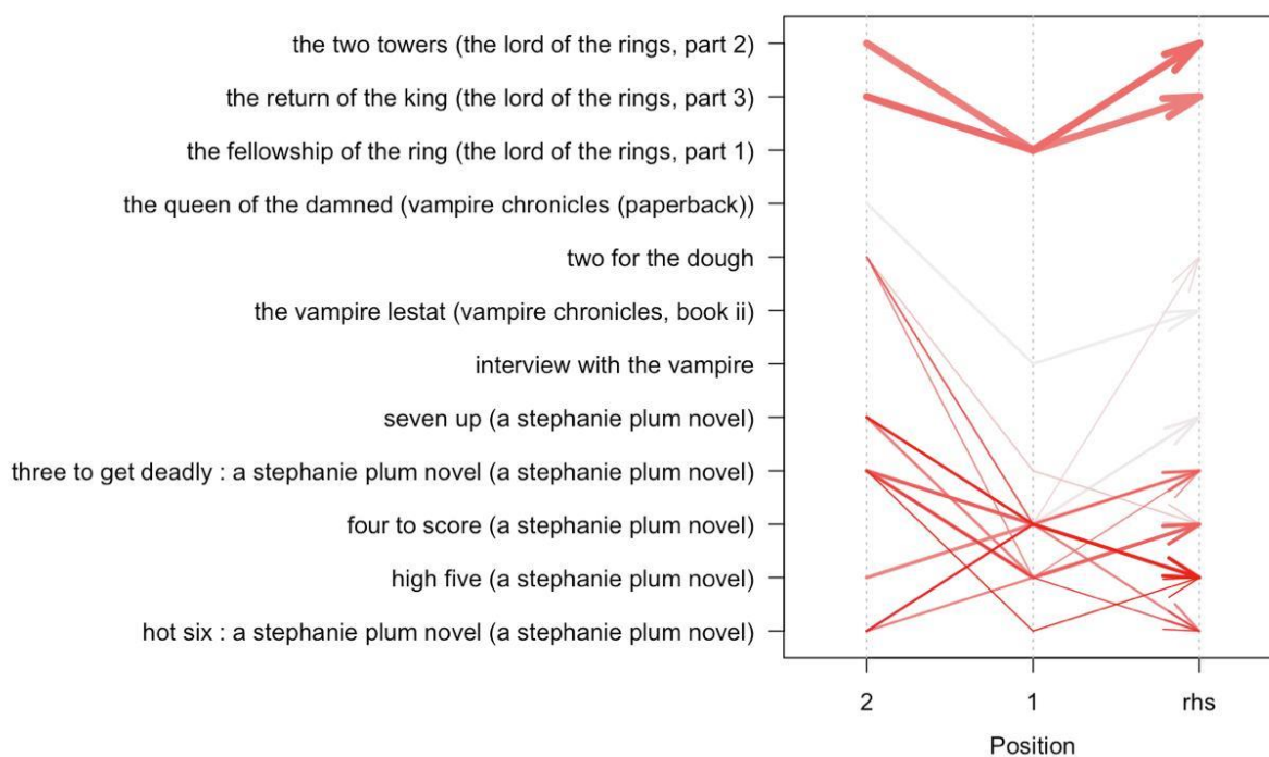
Parallel coordinates plot for 20 rules
